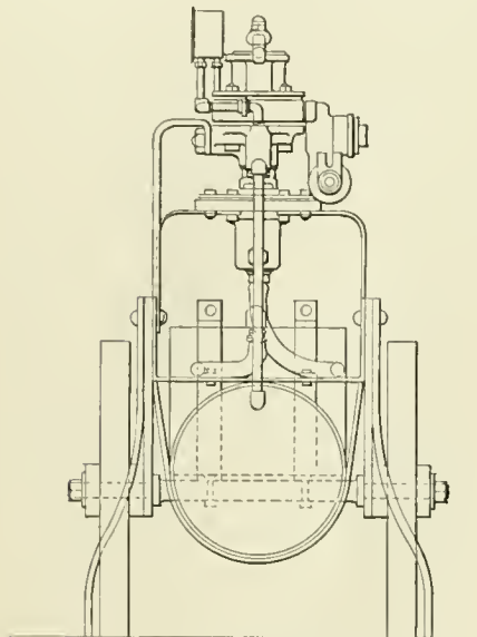
END VIEW OF TRIPLE VALVE TESTING DEVICE.
